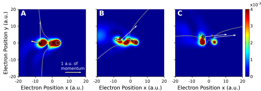
FIG. 4 (color online). Snapshots of the calculated electron density in H_2^+ under a circularly polarized laser pulse at t = t_1 = -1.3 \times 10^{-4} laser cycles (a), t = t_2 = 0.13 laser cycles (b), and t = t_3 = 0.23 laser cycles (c). Time zero is set at a maximum of the x component of the electric field. The gray solid and dashed lines are the contour lines of the potential at the field free energies of the ground and first excited states, respectively. The + signs mark the saddle points of the instantaneous potential. The bold white arrow with a black edge indicates the initial momentum \mathbf{p}_i at the origin of the arrow, and the thin white arrow indicates q_e \mathbf{A}(t) . The two protons are placed at (x, y) = (\pm 3.5 \text{ a.u.}, 0) .
