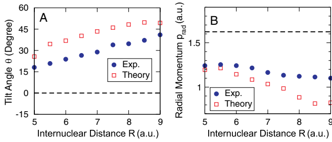
FIG. 2 (color online). Dependence of the tilt angle (a) and the mean radial momentum (b) on R . Dashed lines, predictions of the simple quasistatic model; blue filled circles, experimental data; red open squares, results of TDSE calculations.
