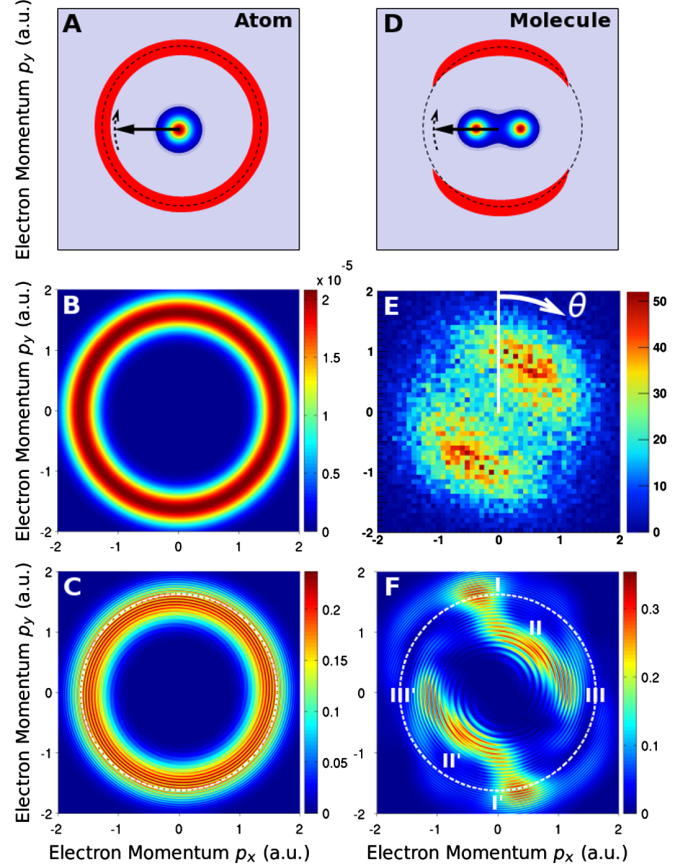
FIG. 1 (color online). Photoelectron momentum distribution from an atom (a)–(c) and a molecule (d)–(f) in a circularly polarized laser pulse at 6 \times 10^{14} W/cm 2 . (a) Expected ring distribution with the radius given by the maximum value of the vector potential A_0 for an atom (dashed line), (b) predictions of the quasistatic ionization theory [23], and (c) result of a TDSE simulation for a two-dimensional model of \text{He}^+ atom. (d) Expected distribution for emission from \text{H}_2^+ , (e) experimental result for \text{H}_2^+ integrated over the internuclear distance R and p_z , and (f) result of a TDSE simulation for a two-dimensional model of \text{H}_2^+ at R = 7 a.u. Contributions I, II, and III (and I', II', III') correspond to three different ionization events (see the text).
