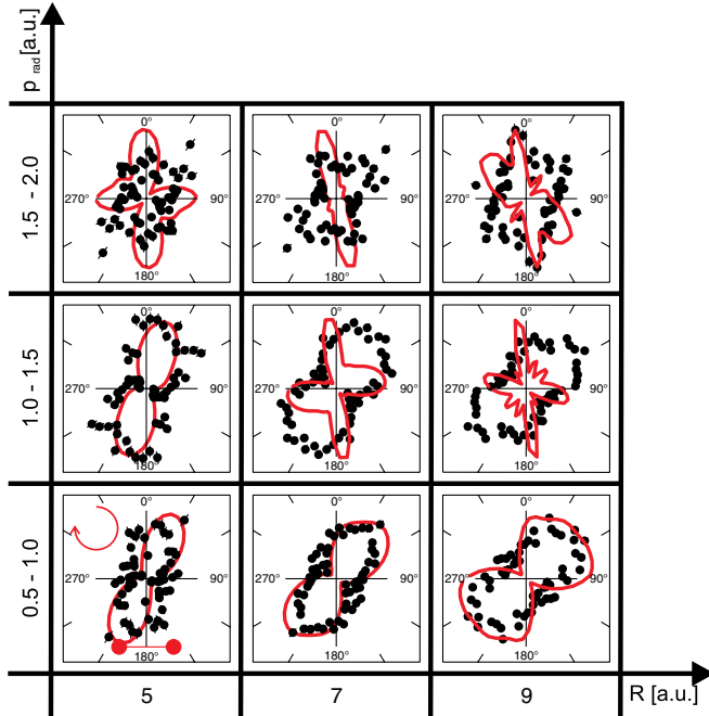
FIG. 3 (color online). Angular distributions of the experimental data (black dots) and theoretical results (red solid line) for a clockwise circularly polarized laser pulse of intensity 6 \times 10^{14} W/cm 2 . The experimental data are integrated over p_z . The internuclear axis is set along the x axis. The columns correspond to R = 5 a.u., R = 7 a.u., and R = 9 a.u. from left to right, and the rows to different regions of electron radial momenta.
